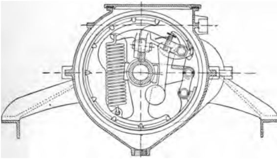
FIG. 244.—Mechanism of the Expanding Ring Clutch of the Columbia Light Car.
